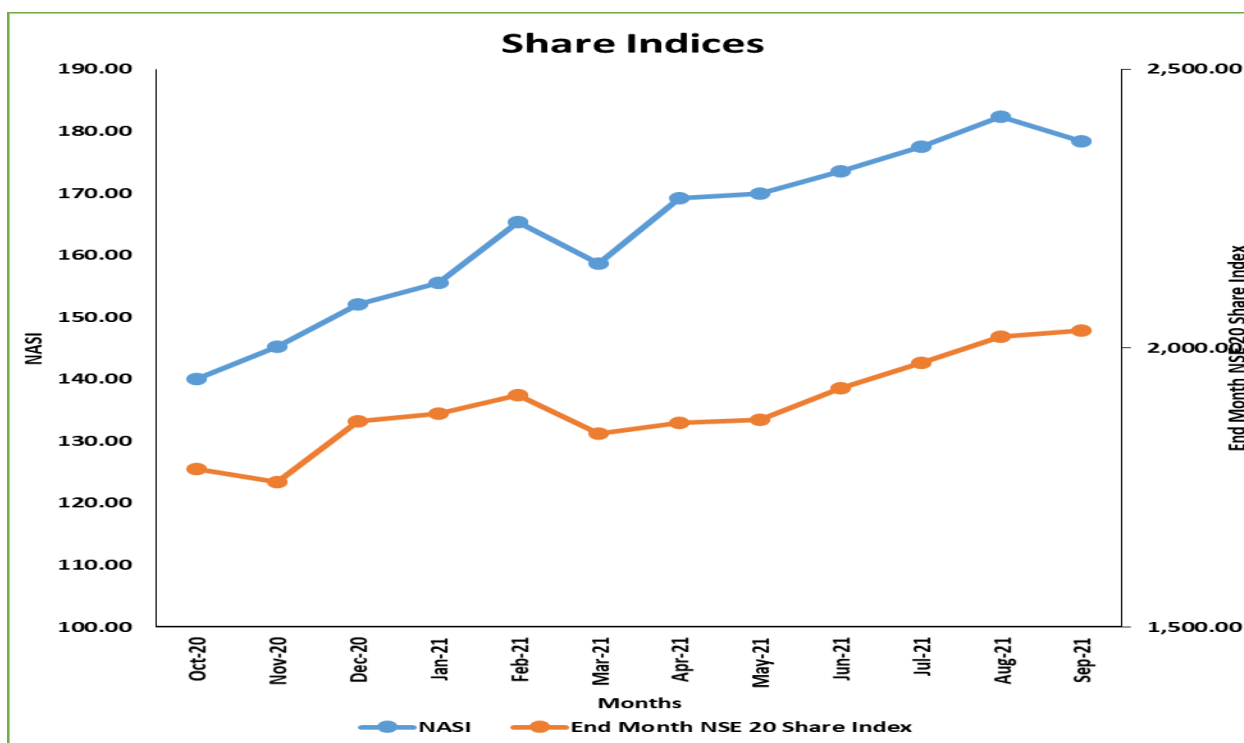
Figure 7: Trend in Share Indices
